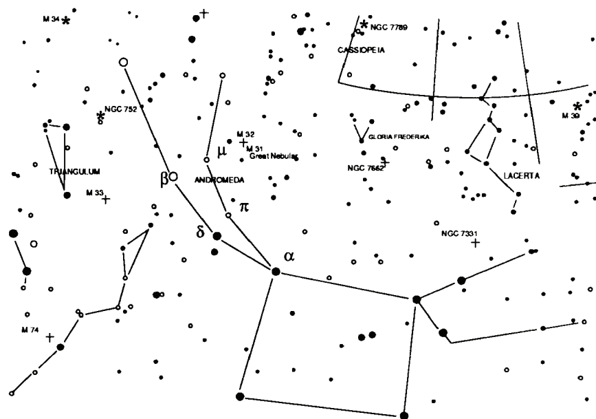
Fig. 16 Andromeda Galaxy
